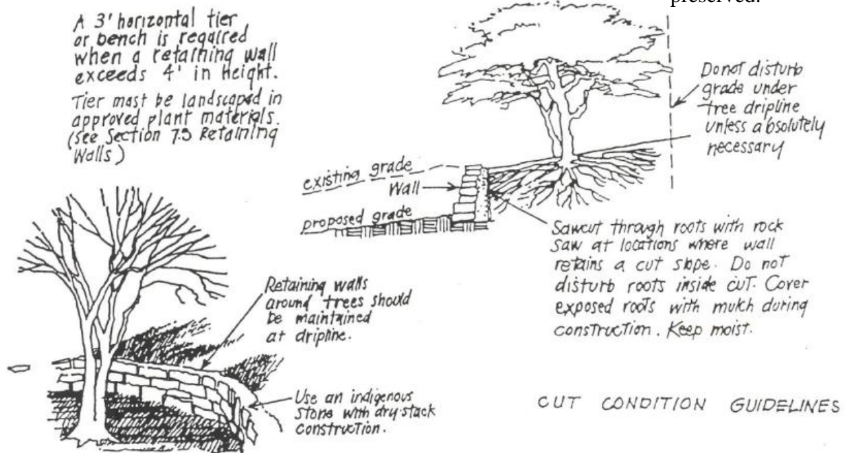
TREE WELL RETAINING WALL
