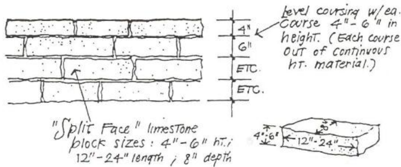
LIMESTONE MASONRY WALL ELEVATION
