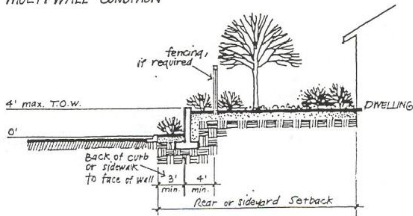
SINGLE WALL CONDITION
